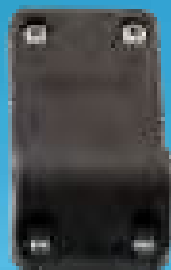
1023 TILT-UP MOUNTING BRACKET Extra mounting bracket for all Scotty tilt-up Downriggers. Also used as the mounting bracket for the Scotty 2500 Line Puller. Dimensions: 2 1/2" x 4 1/2" Bolting dimensions: 3 3/4" x 1 5/8"
